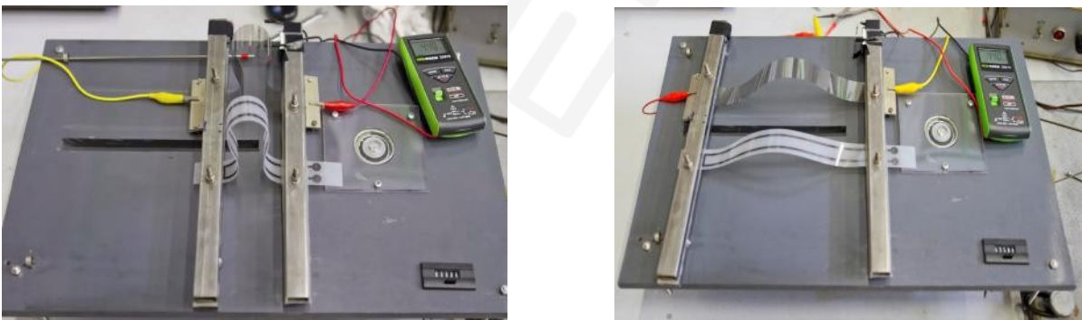
Figure 2: Fatigue test on graphene coated PET, sheet resistance measure before (left) and after (right) more than 50.000 cycles.
