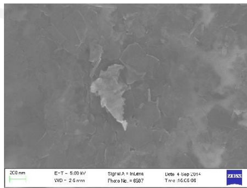
Figure 3: Scanning electronic microscopy on PET film coated with graphene flakes
